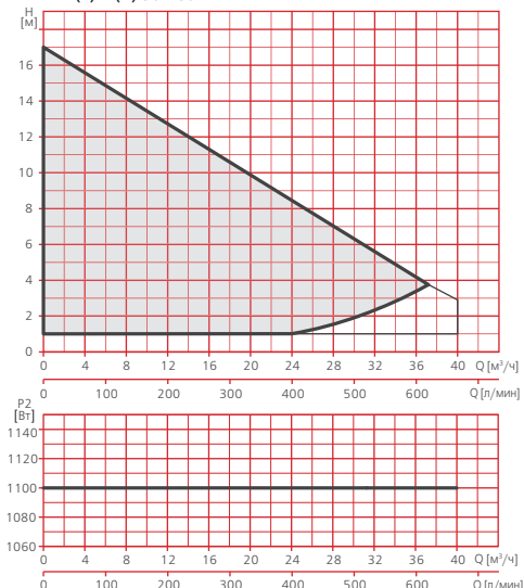
RV1(2)-F (X) 50-180
