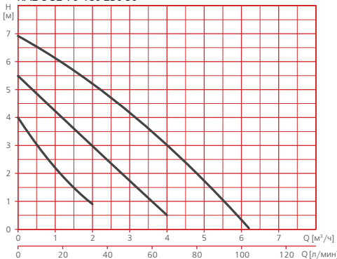
RA2-S 32-70-180 230 50
