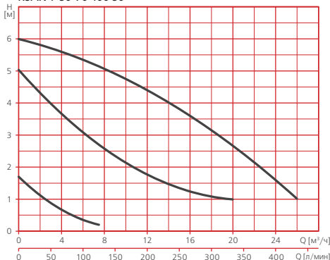
RSAN-F 50-70 400 50
