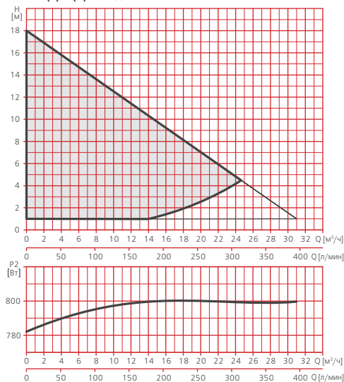
RV1(2)-F (X) 40-180
