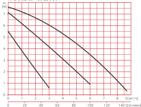
RA2-S 32-80-180 230 50
