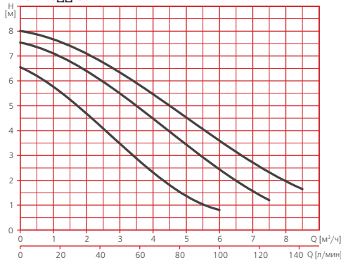
RSAN-S 3 -80
